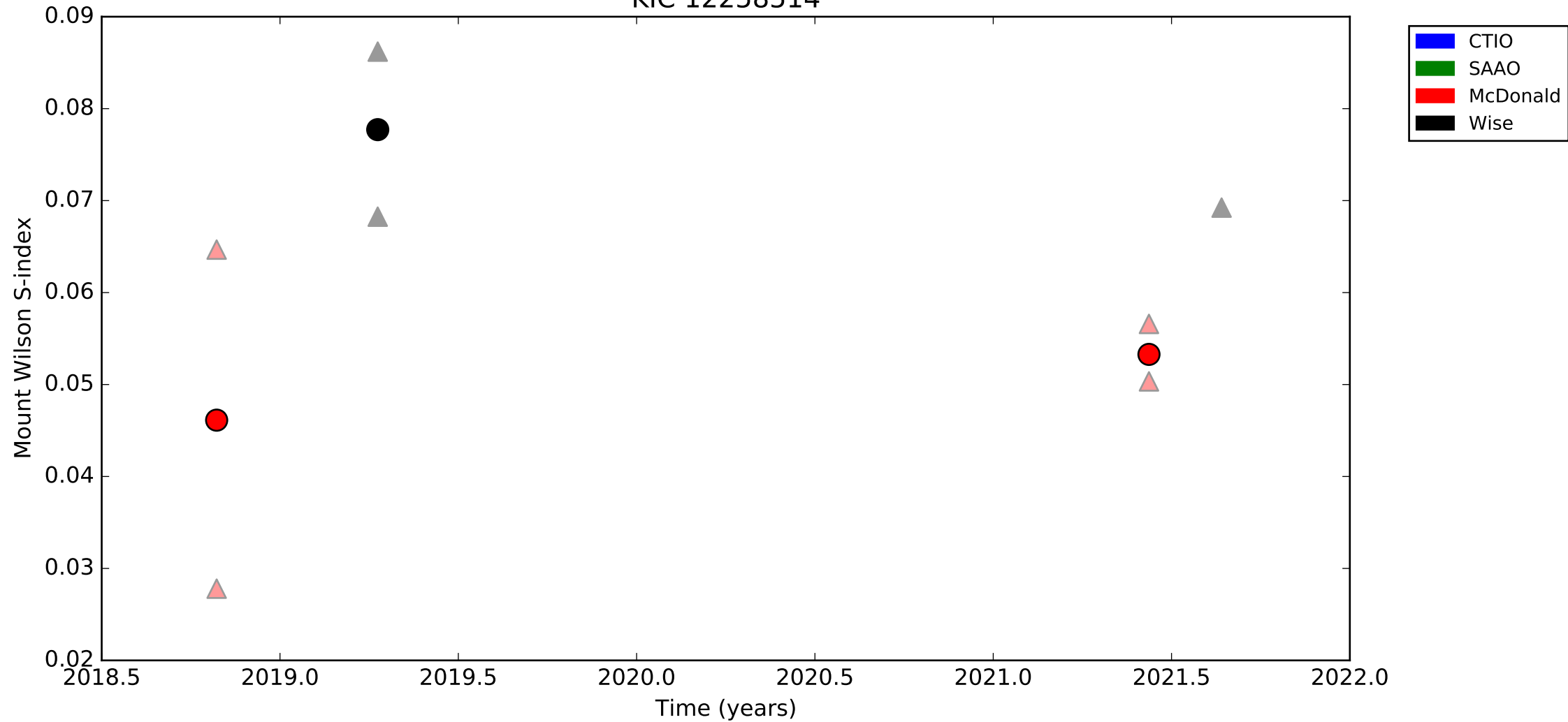
KIC 12258514
