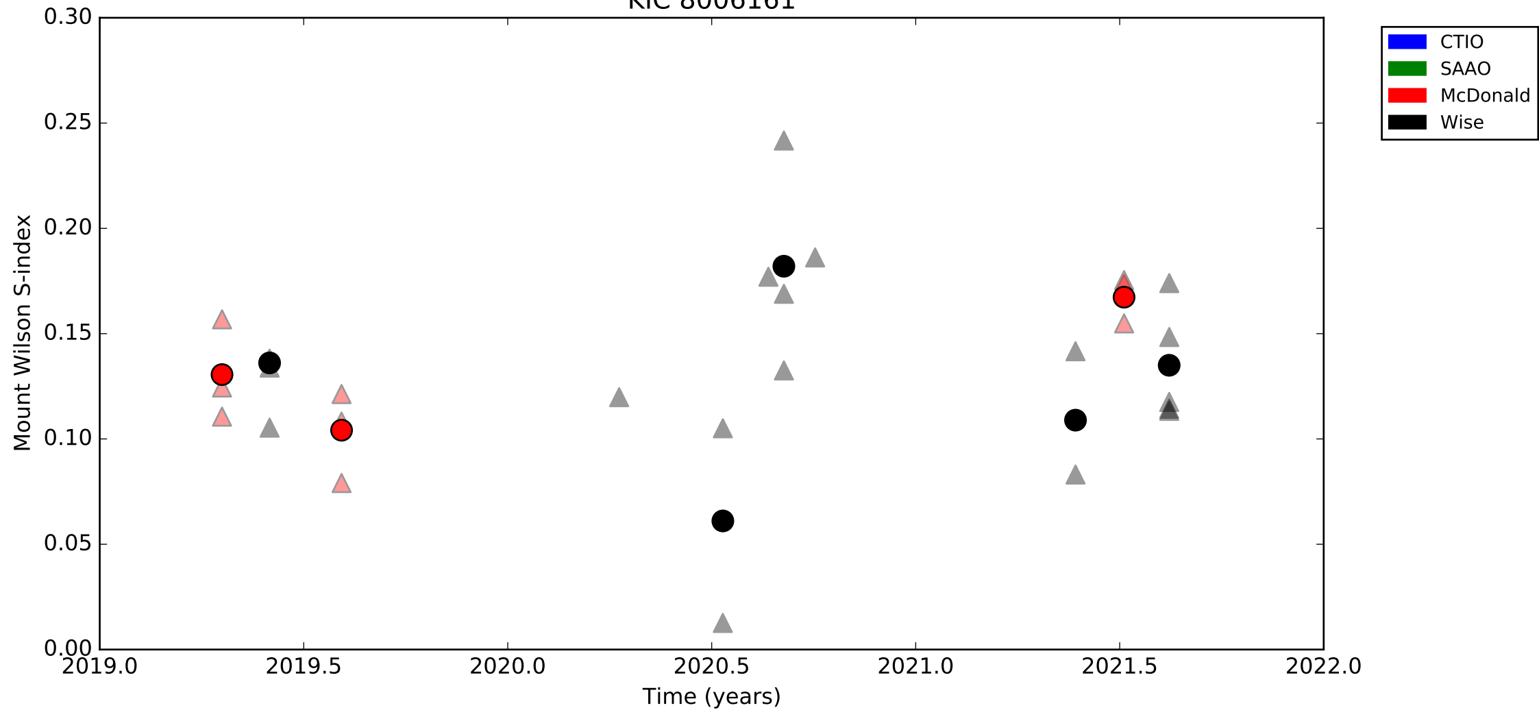
KIC 8006161
