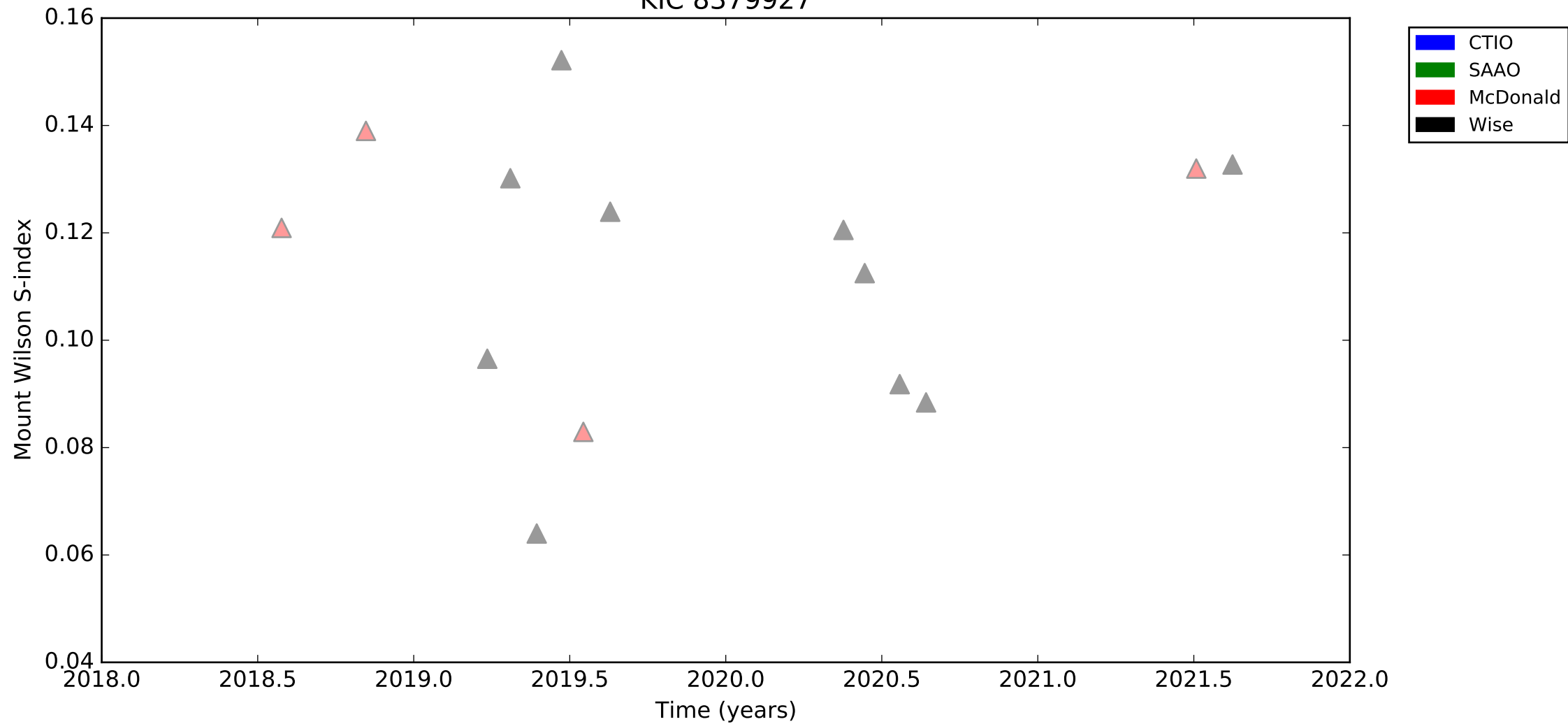
KIC 8379927
