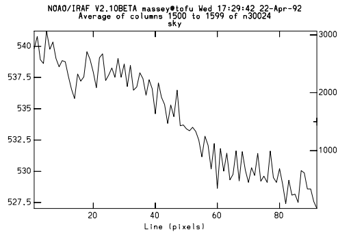
Figure 14: The cut along the spatial axis of a long program exposure appears to be consistent with a cut along the spatial axis of a bright twilight sky exposure: there is a 2% gradient from one side of the chip to the other.
